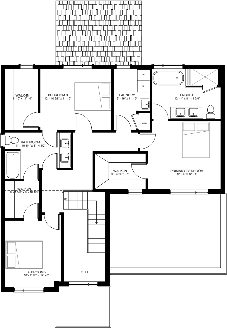
SECOND FLOOR 1158 SQ.FT.
