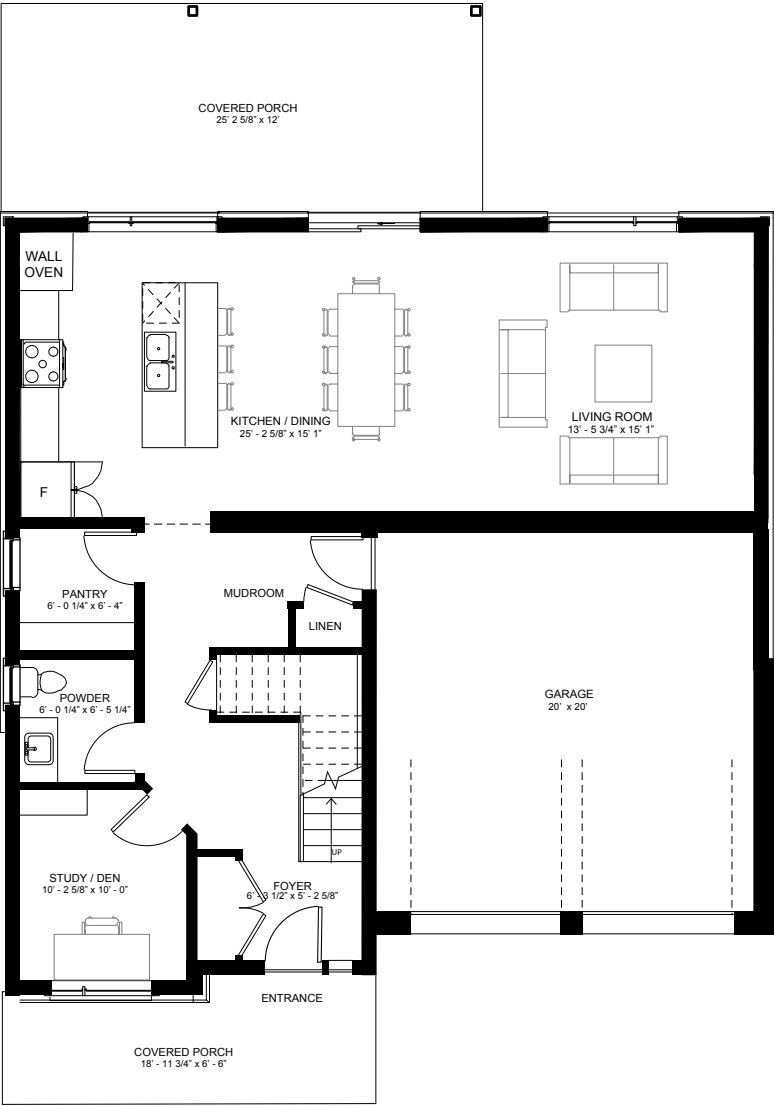
MAIN FLOOR 1136 SQ.FT.
