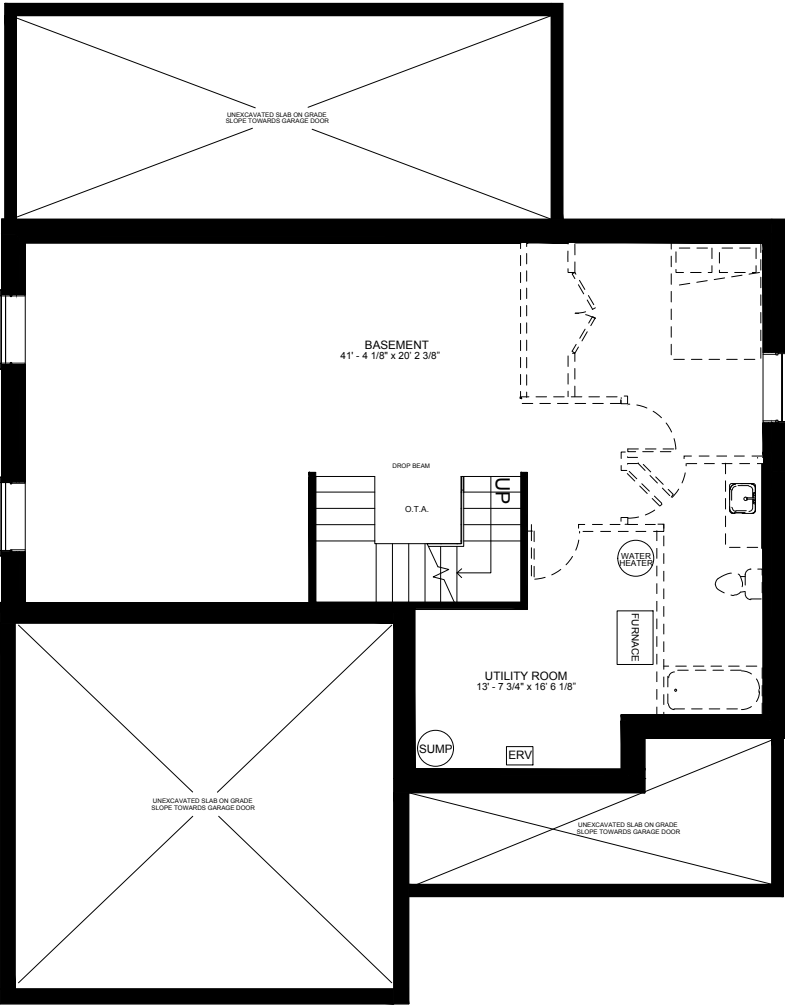
OPTIONAL FINISHED BASEMENT 916 SQ.FT
