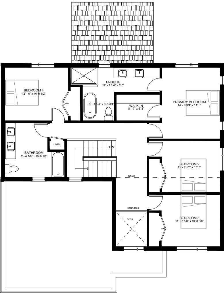
SECOND FLOOR 1202 SQ.FT.
