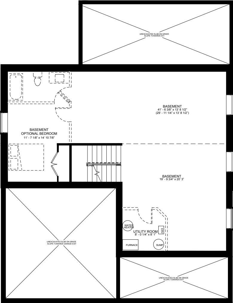
OPTIONAL FINISHED BASEMENT 1154 SQ.FT.
