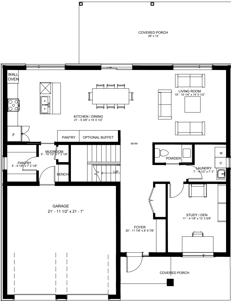
MAIN FLOOR 1317 SQ.FT.
