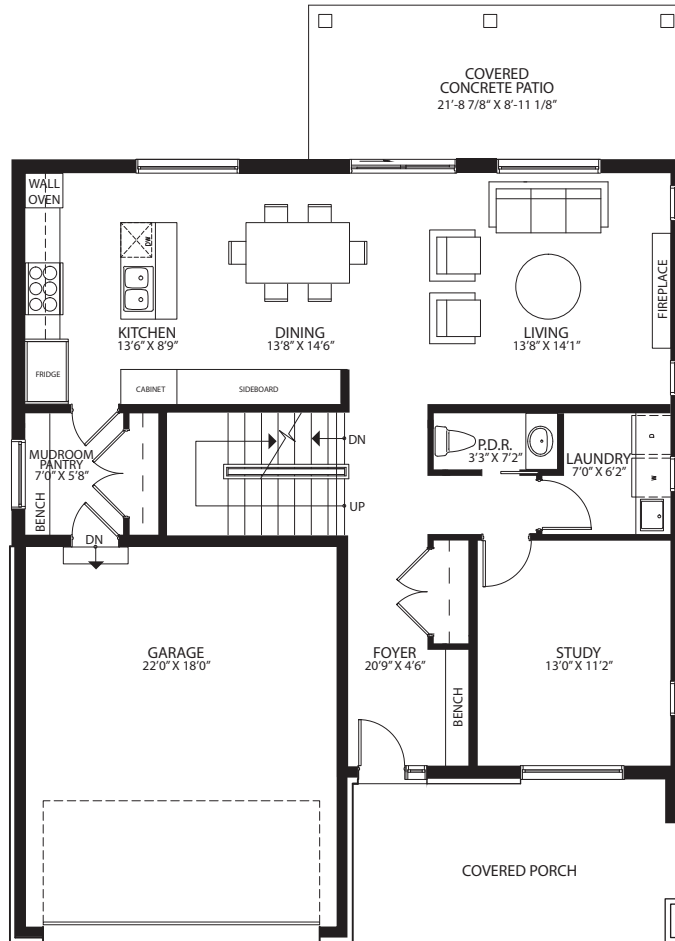
MAIN FLOOR 1151.4 SQ. FT.
