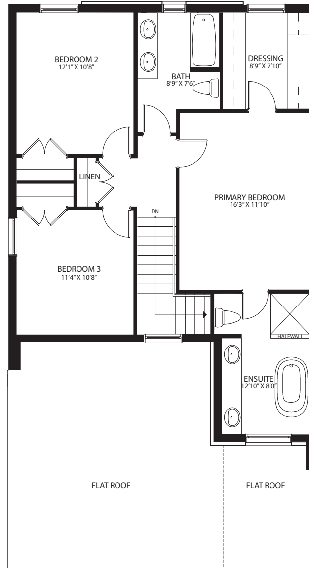
SECOND FLOOR 975 SQ. FT.
